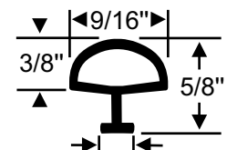
70-4067-245 • per/ft.
