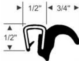
Fits flanges 3/16" to 1/4" 70-3593-99 - 25ft. Strip
