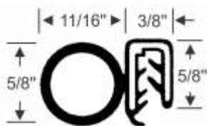
Fits flanges up to 1/8" 70-3584-99 • per/ft.
