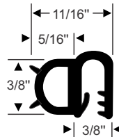
Fits flanges 3/64" to 1/8" 70-3855-99 • per/ft.
