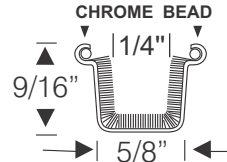
FLEXIBLE METAL SPINE 70-1238-135 - 5' strip 70-1239-135 - 6' strip
