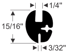
60-0082-119 • per/ft. USES 60-0607-119 LOCKSTRIP
