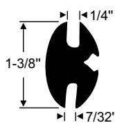
70-4299-119 • per/ft. USES 60-0607-119 LOCKSTRIP
