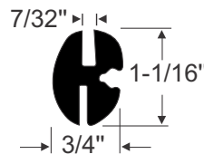
40-0496-119 • per/ft. USES 30-0439-119 LOCKSTRIP
