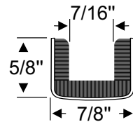
FLEXIBLE METAL SPINE 60-0375-135 - 5' strip 60-0129-135 - 90" strip
